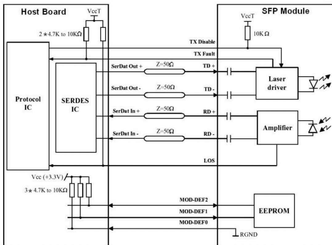
Figure 5. SFP Host Recommended Circuit
